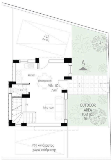
Ground Floor Plan for Villa
