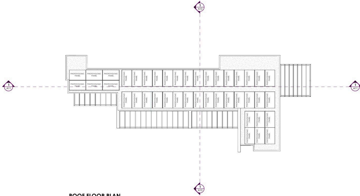
ROOF FLOOR PLAN 1 : 100
