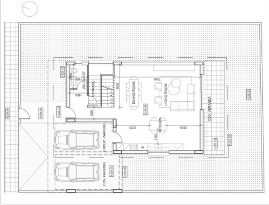
HOUSE C2 ground floor plan
