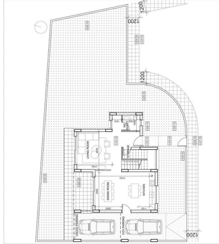
HOUSE A2 ground floor plan
