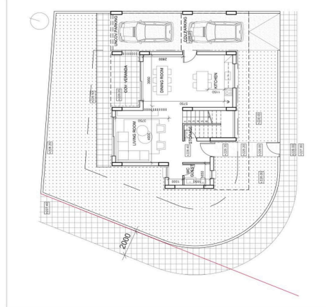
HOUSE A1 ground floor plan
