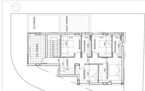
floor plan
