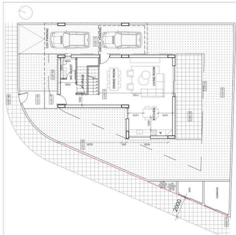
HOUSE B ground floor plan
