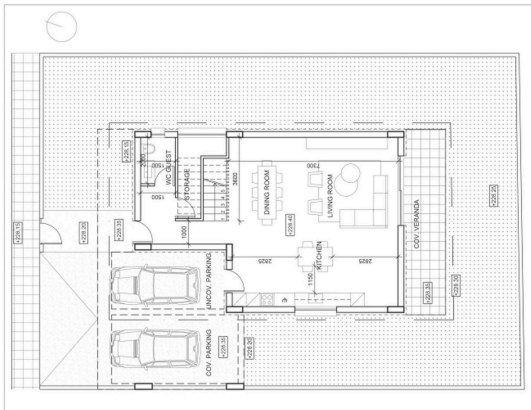
HOUSE C2 ground floor plan
