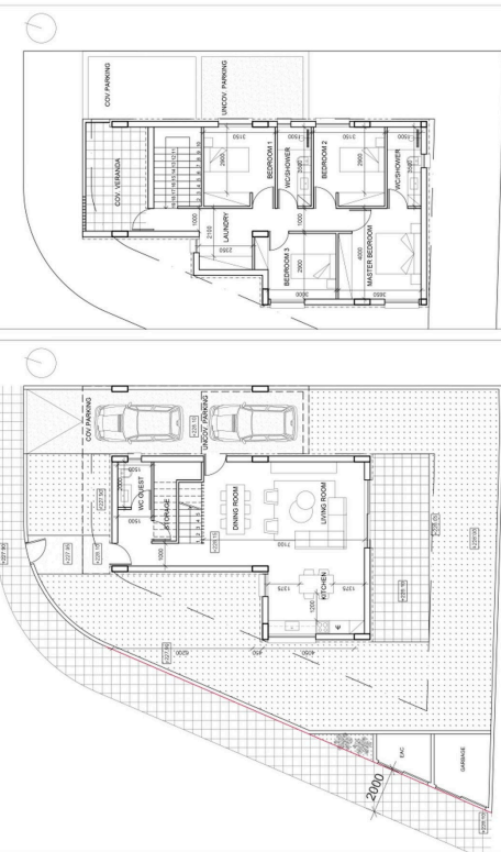
HOUSE B ground floor plan
