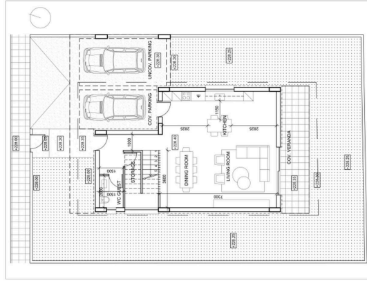
HOUSE C1 ground floor plan
