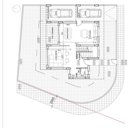
HOUSE A1 ground floor plan
