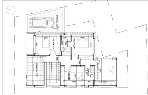
floor plan
