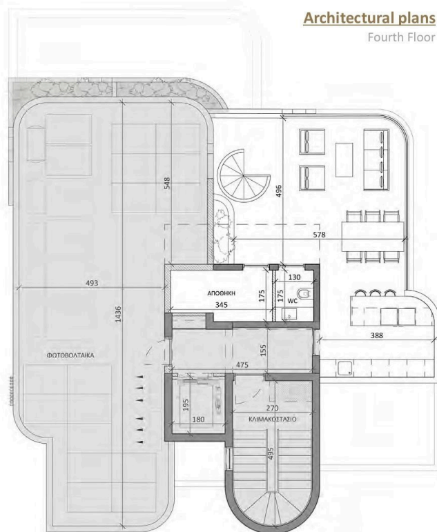
Penthouse 301—Fourth Floor
