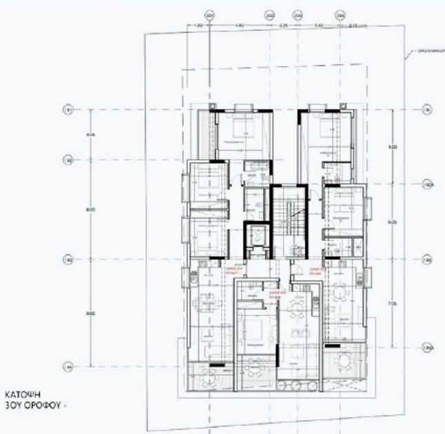
3rd FLOOR
