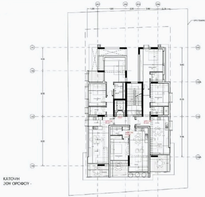
2nd FLOOR
