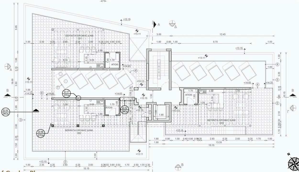
Roof Garden Plan
