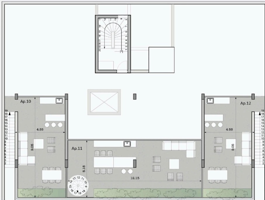
ROOF GARDEN
