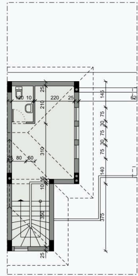
ATTIC FLOOR PLAN
