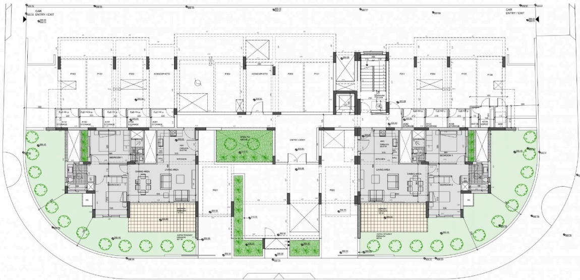
GROUND FLOOR
