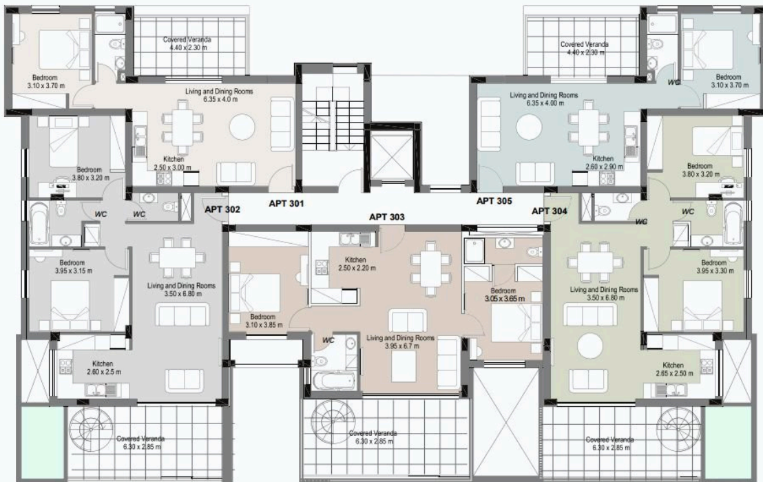
Third Floor
