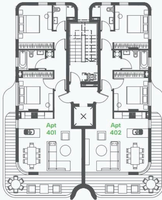
FLOOR 4
