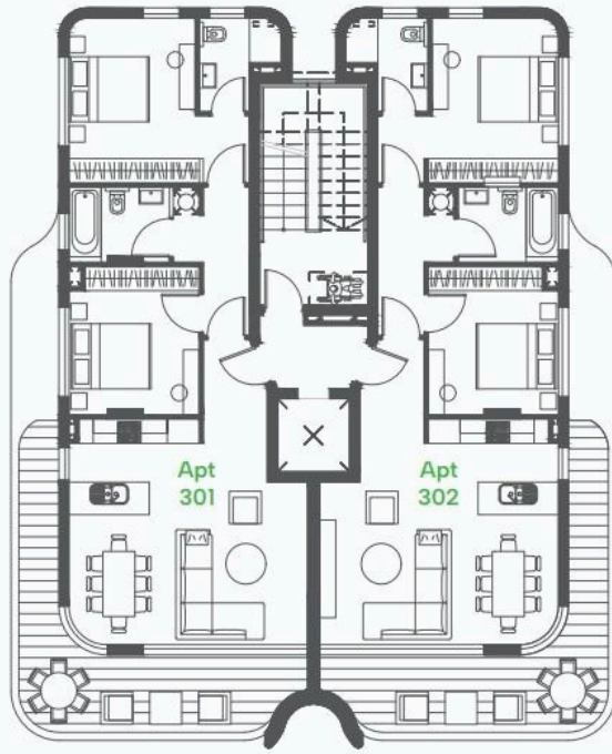
FLOOR 3
