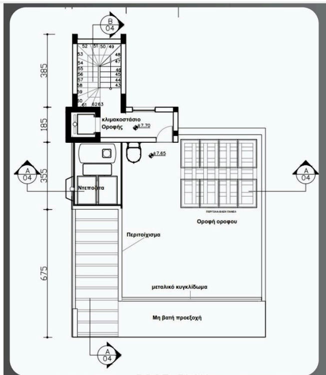
ROOF PLAN
