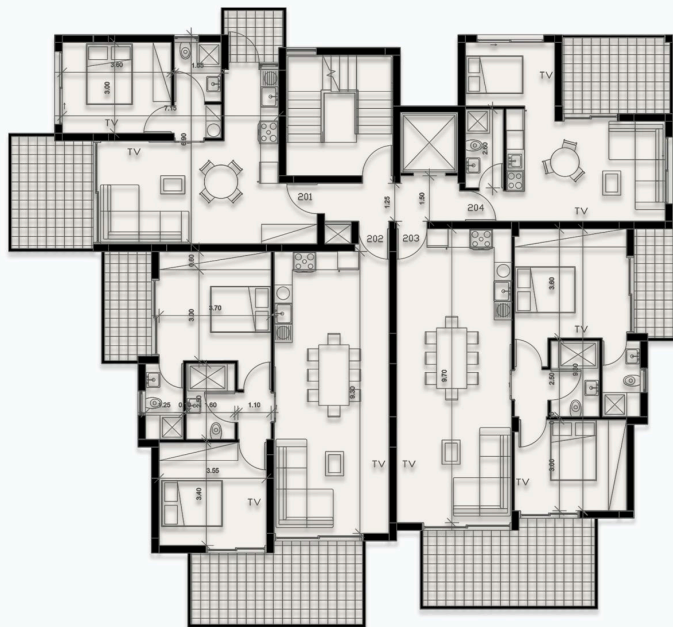
SECOND FLOOR
