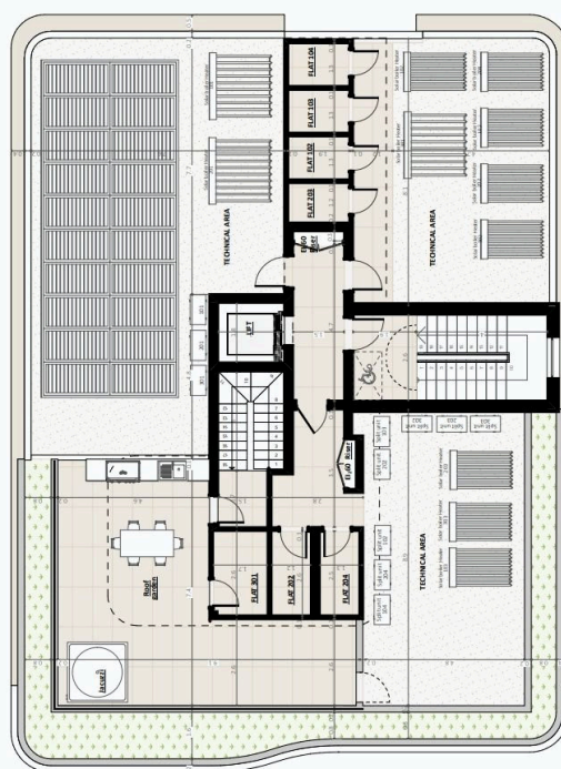
ROOF GARDEN
