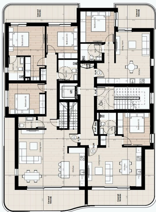
THIRD FLOOR
