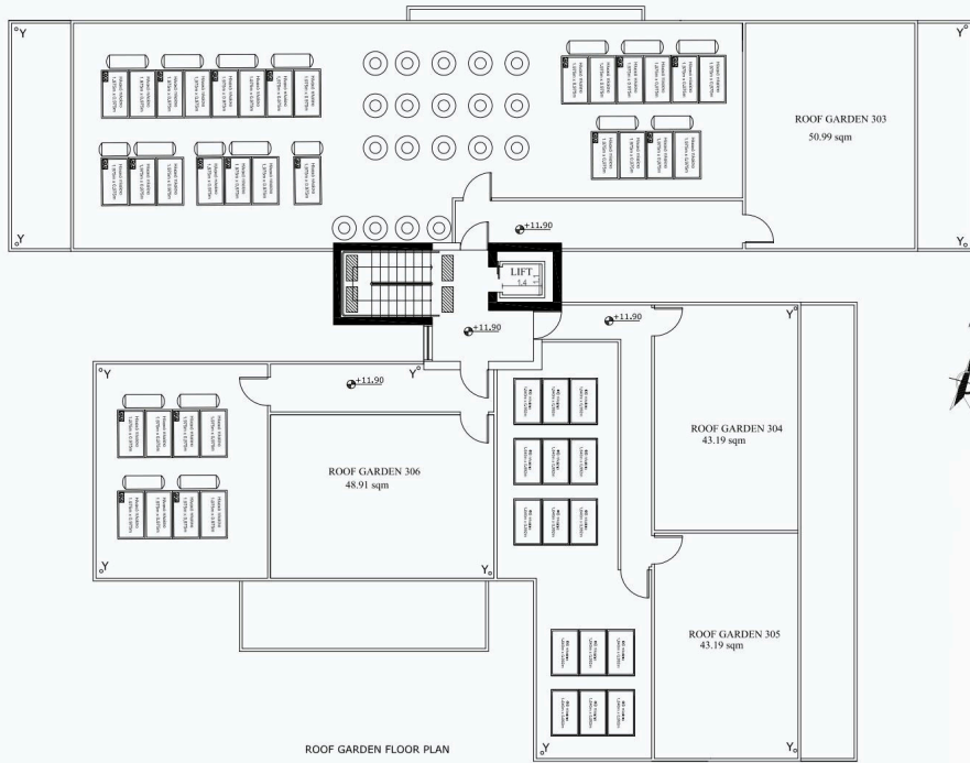
ROOF GARDEN FLOOR PLAN
