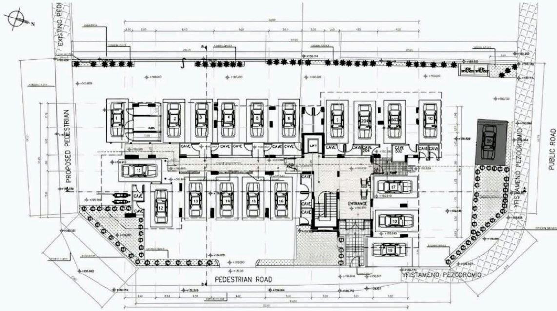
Parking Plan
