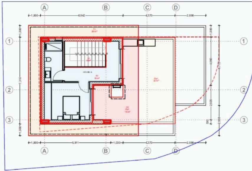
HOUSE A SECOND FLOOR
