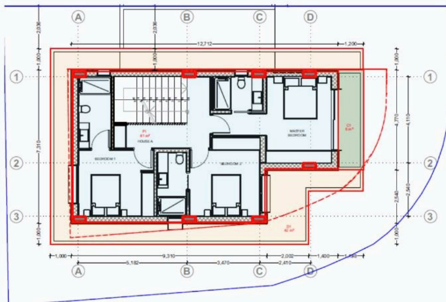
HOUSE A FIRST FLOOR
