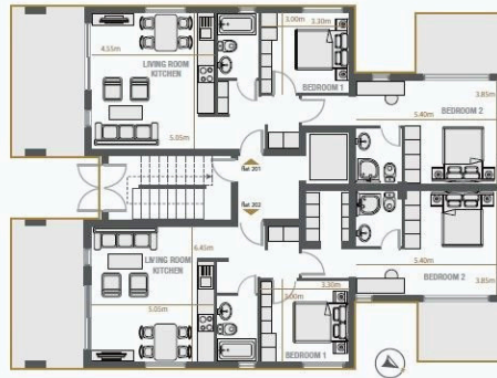
2nd Floor
