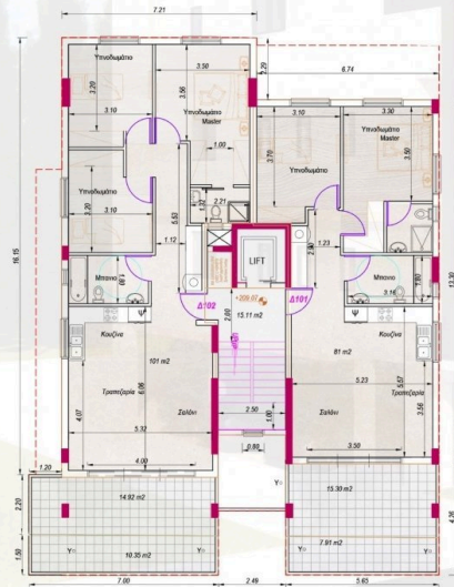
1 & 2 ΟΣ ΟΡΟΦΟΣ - FIRST & SECOND FLOOR
