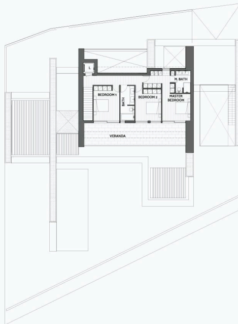
VILLA 02 FIRST FLOOR
