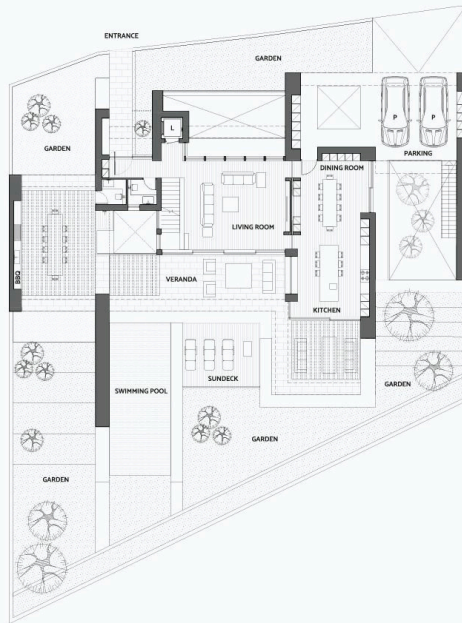
VILLA 02 GROUND FLOOR
