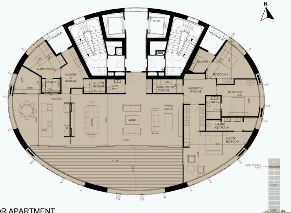
FLOOR APARTMENT
