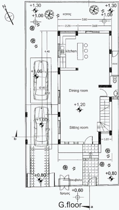
house 2 type 2
