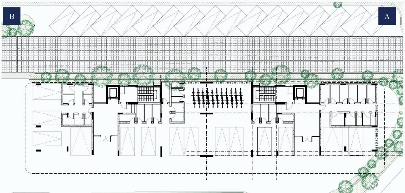
BUILDINGS A & B GROUND FLOOR
