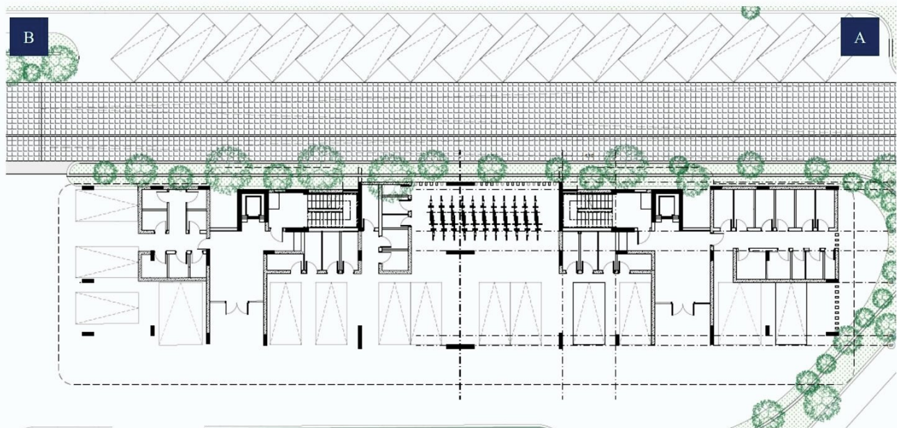
BUILDINGS A & B GROUND FLOOR
