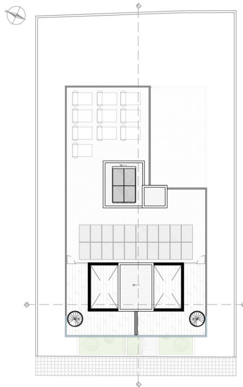
ROOF FLOOR PLAN
