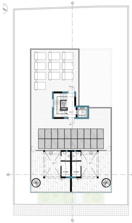
ROOF FLOOR PLAN
