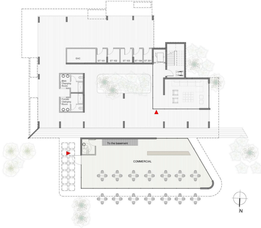
A001-BLOCK A GROUND FLOOR 1:100
