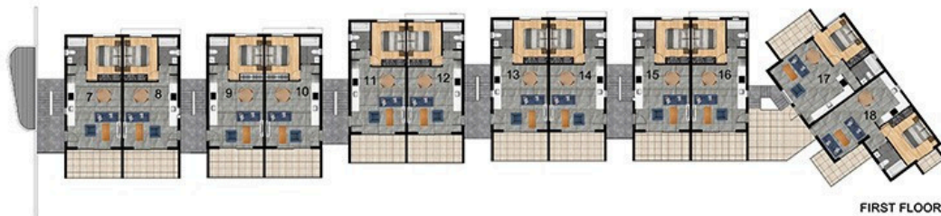
FIRST FLOOR
