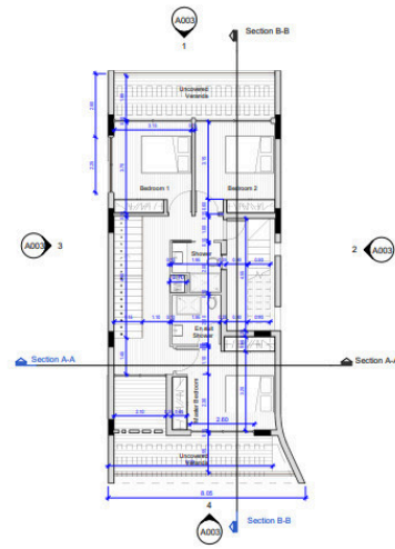
A002 FIRST FLOOR PLAN 1:100
