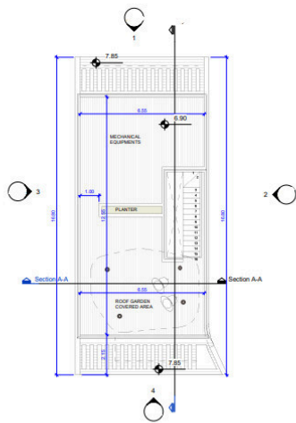
ROOF GARDEN PLAN 1:100
