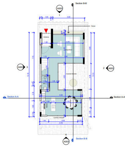
A001 GROUND FLOOR PLAN 1:100
