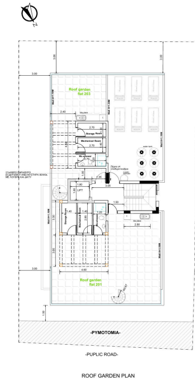
ROOF GARDEN PLAN
