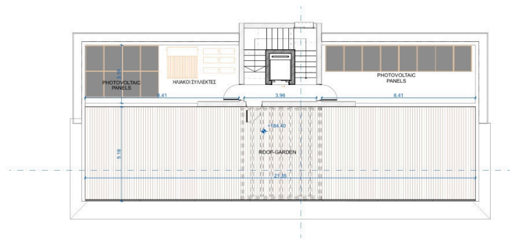
2. ROOF PLAN 1:100
