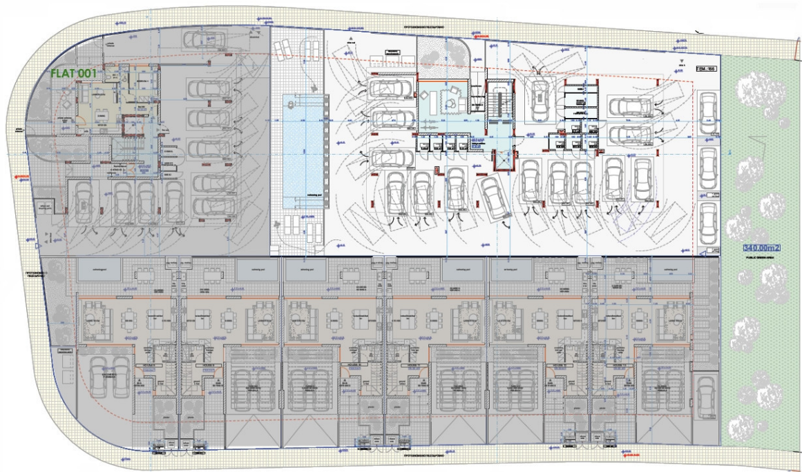
BUILDING B - GROUND FLOOR
