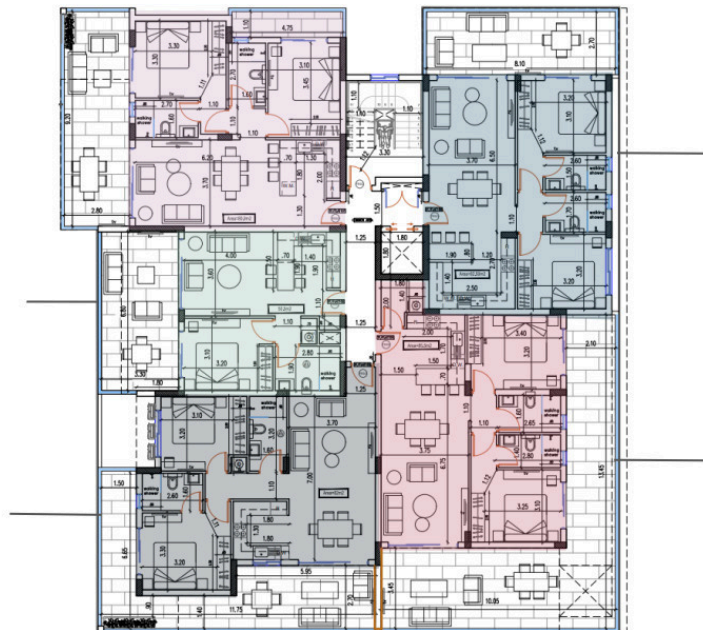
FLOORPLANS – FIRST FLOOR
