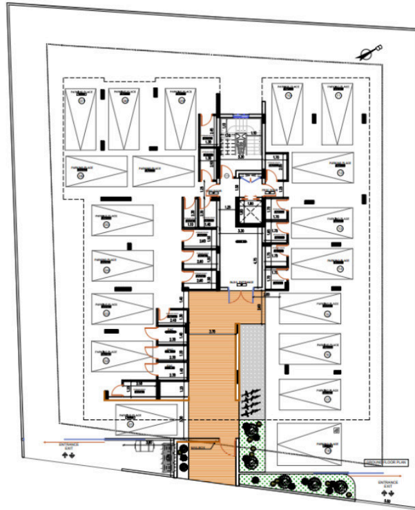
FLOORPLANS – GROUND FLOOR
