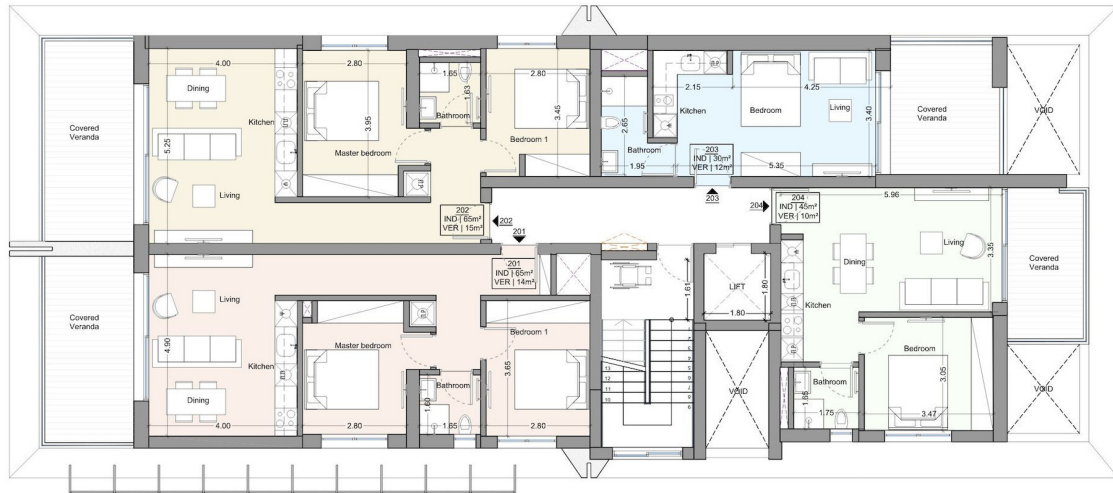
2nd Floor
