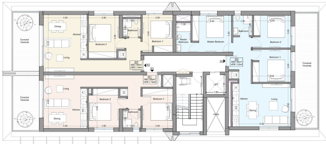
3rd Floor
