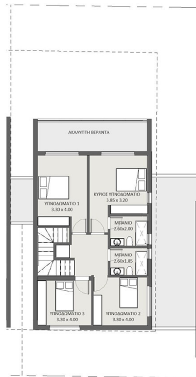
FLOOR PLANS - FIRST FLOOR
