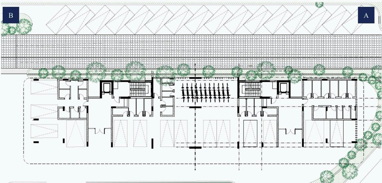
BUILDINGS A & B GROUND FLOOR
