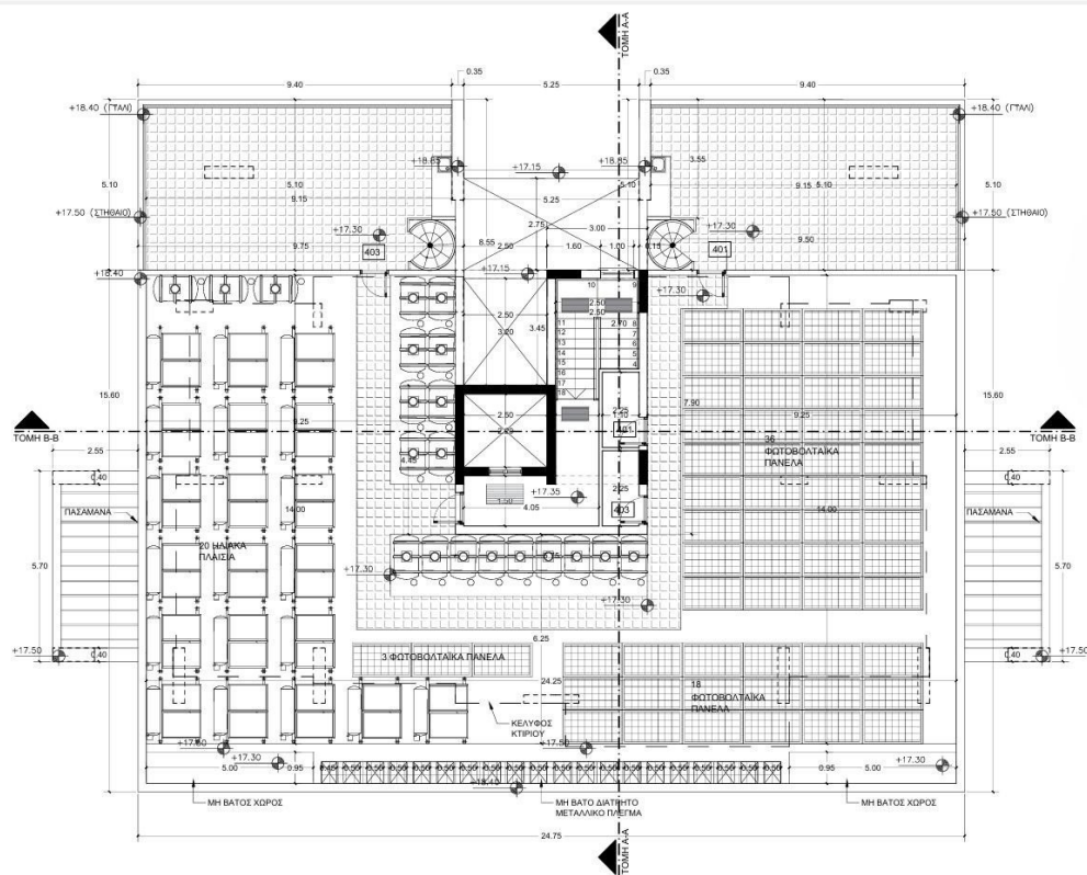
ROOF PLAN
