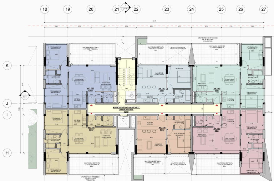
1 C_First Floor 1:100
