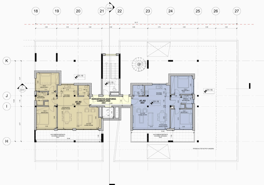
1 C_Roof Terrace 1:100
