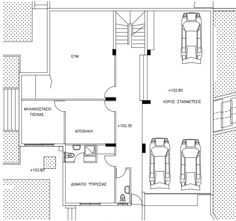
Plans Basement
