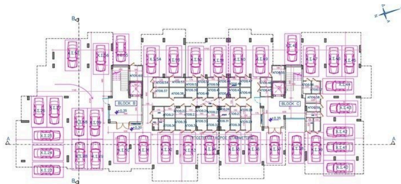
GROUND FLOOR PLAN BLOCK B & BLOCK C
