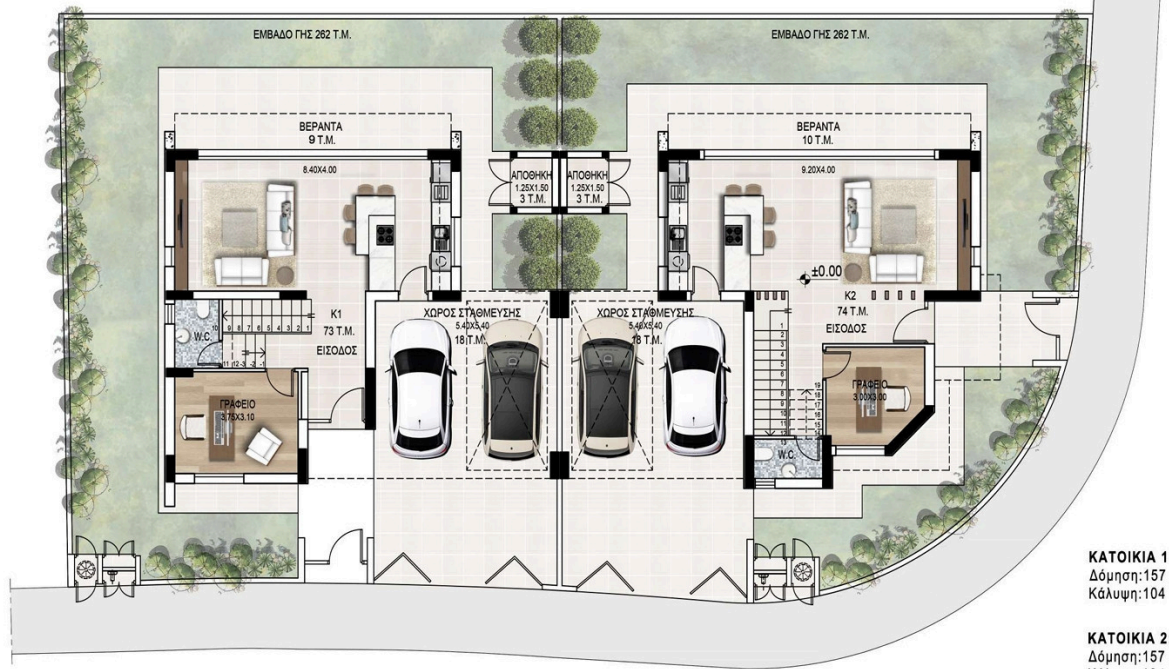
Ground Floor Scale 1:100
