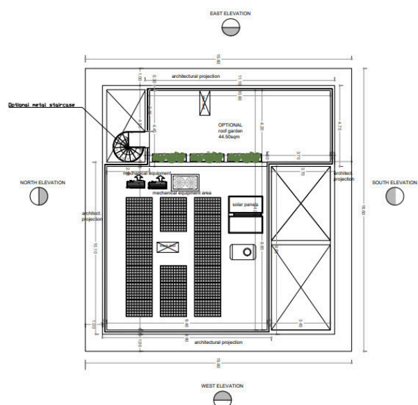
ROOF PLAN
