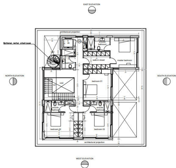
FIRST FLOOR Internal Area: 150.8 sq.m.
