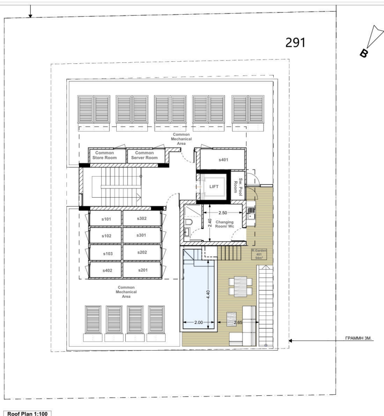
Roof Plan 1:100
