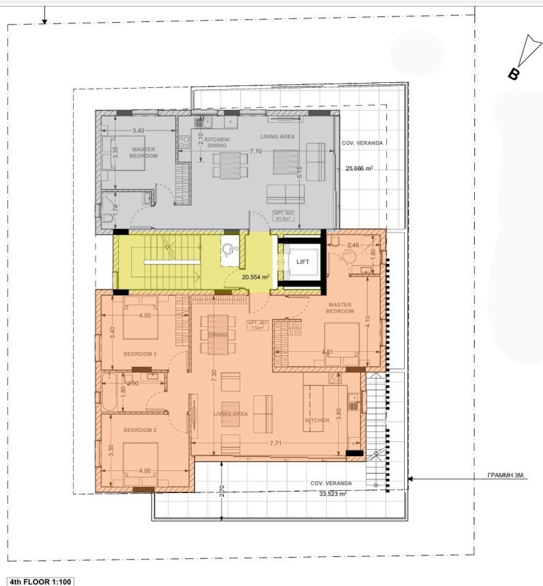
4th FLOOR 1:100
