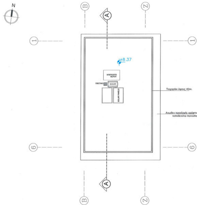
ROOF PLAN
