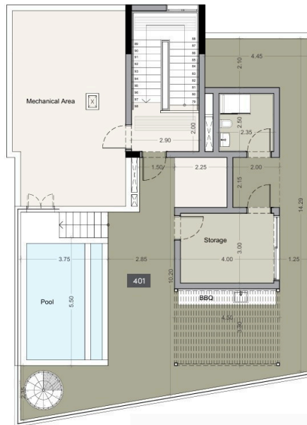
roof terrace
