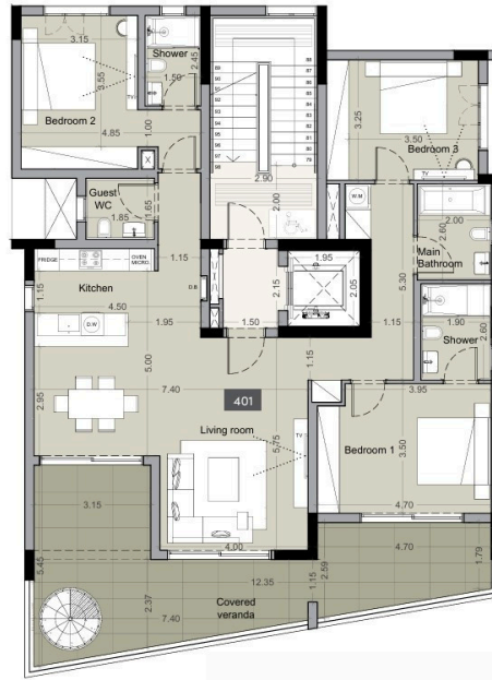
4th floor
