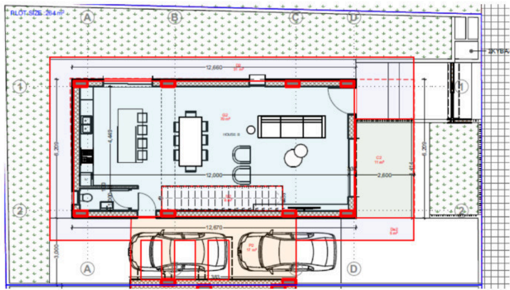
HOUSE B GROUND FLOOR
