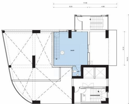
MIDDLE FLOOR PLAN SCALE 1:100
