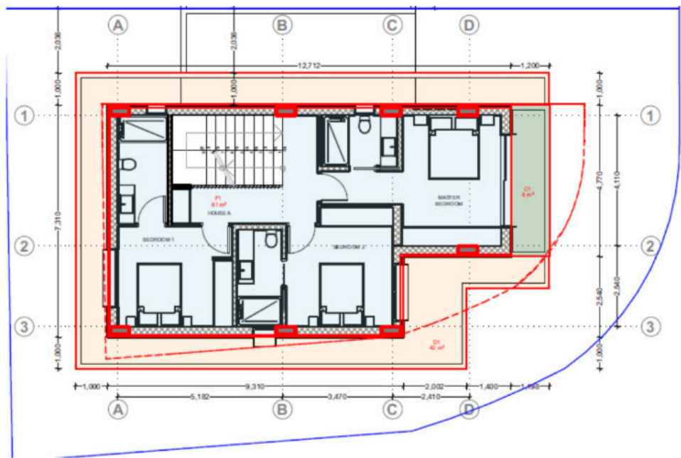
HOUSE A FIRST FLOOR
