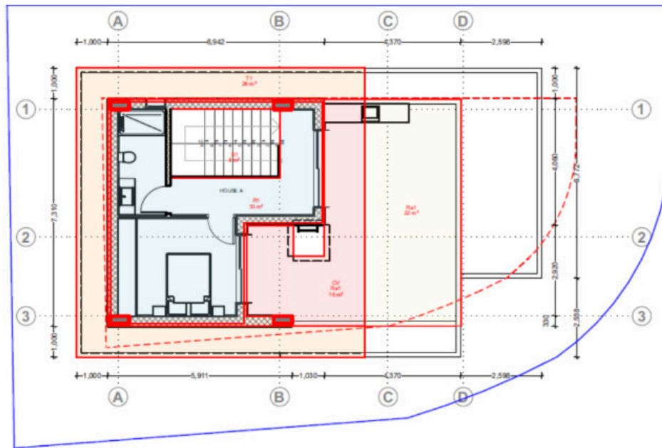
HOUSE A SECOND FLOOR
